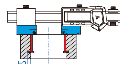
measuring internal groove diameter with spherical measuring face (depth h2 \leq 2.5\text{mm} )
